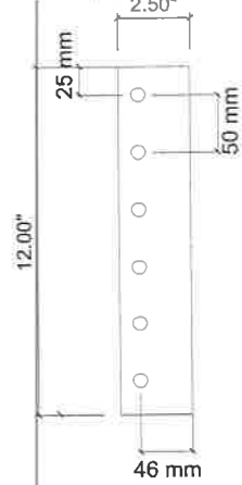
PLAN (Coupling) DETAIL - 1
