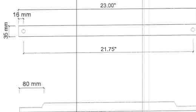
PLAN (Horizontal Braces) DETAIL - 3
