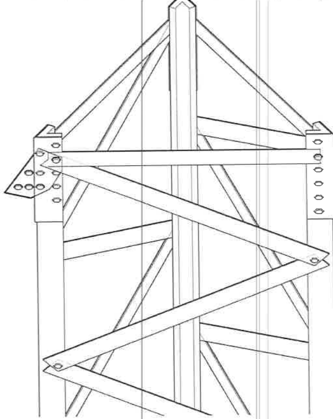
TOP ISOMETRIC
