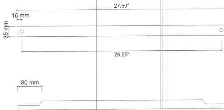
PLAN (Diagonal Braces) DETAIL - 2
